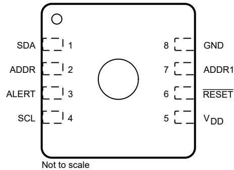
Figure 5-1. HDC302x DEF, DEH, or DEJ Package 8-Pin WSON Top View
